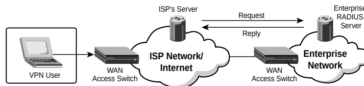
Figure 6 – A common use of Proxy RADIUS is for a server at the service provider's POP to access user profiles on a server at the organization's site.
